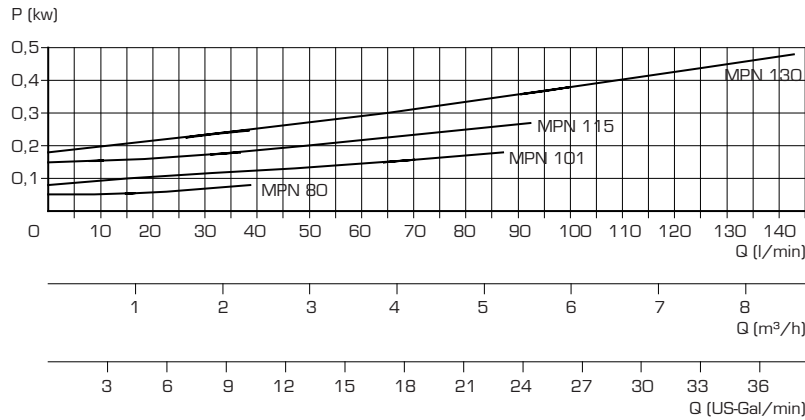
Motor power
