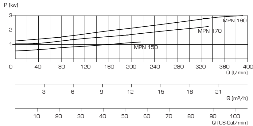
Motor power
